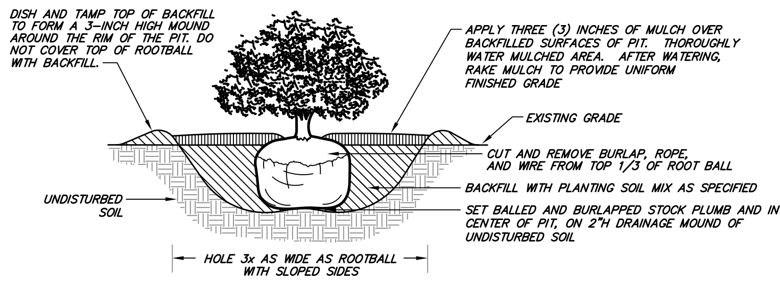
TYPICAL SHRUB PLANTING DETAIL NOT TO SCALE
