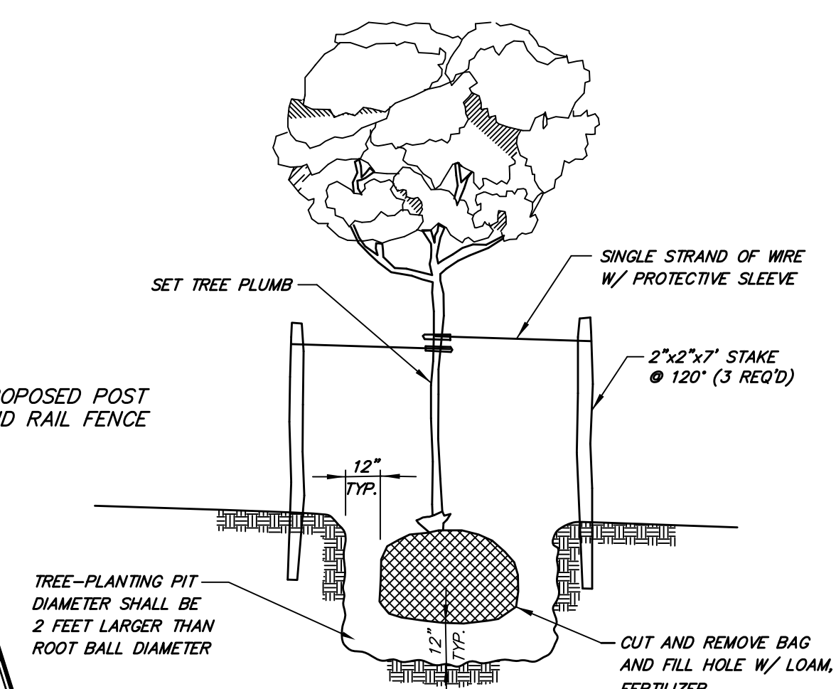
TREE PLANTING CROSS SECTION NOT TO SCALE
