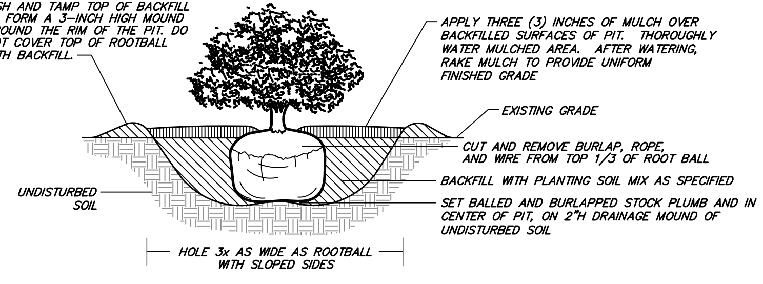
TYPICAL SHRUB PLANTING DETAIL NOT TO SCALE
