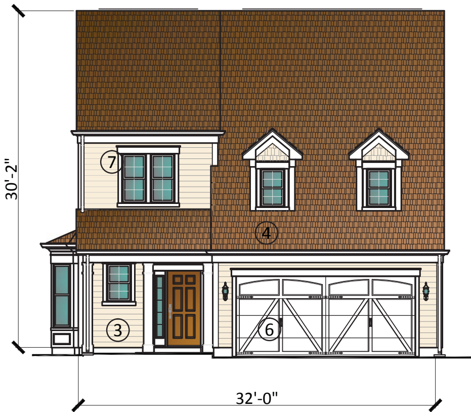
ELEVATION 1 - MILAN
