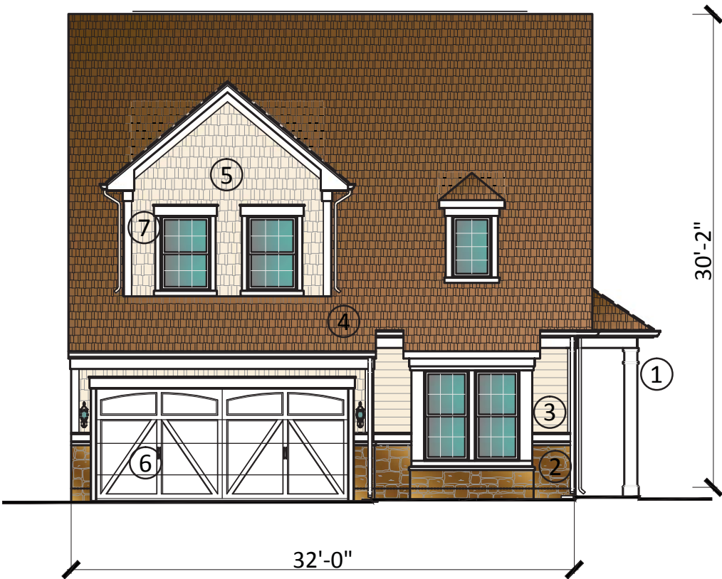
ELEVATION 2 - FLORENCE
