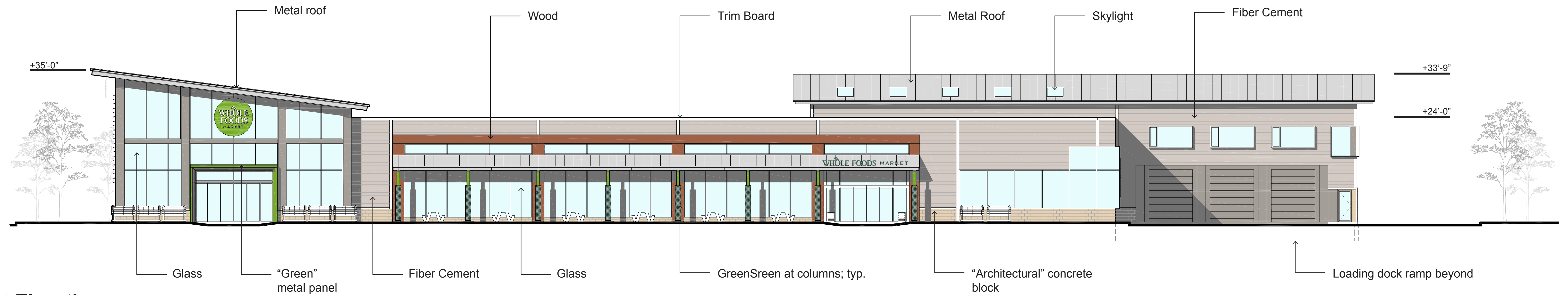
East Elevation
