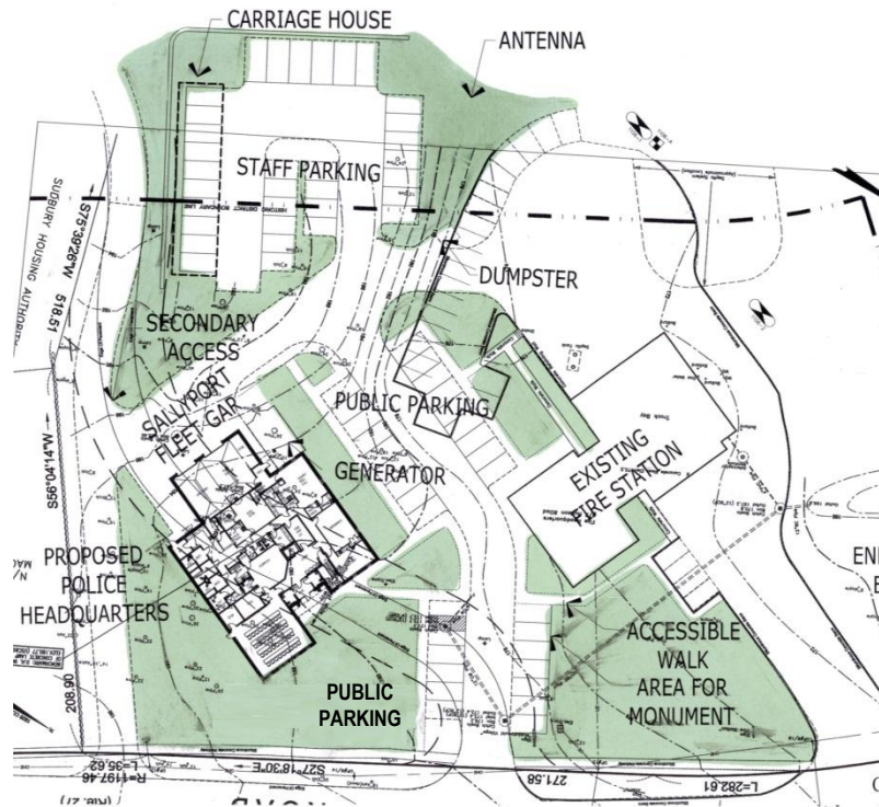
SITE PLAN
